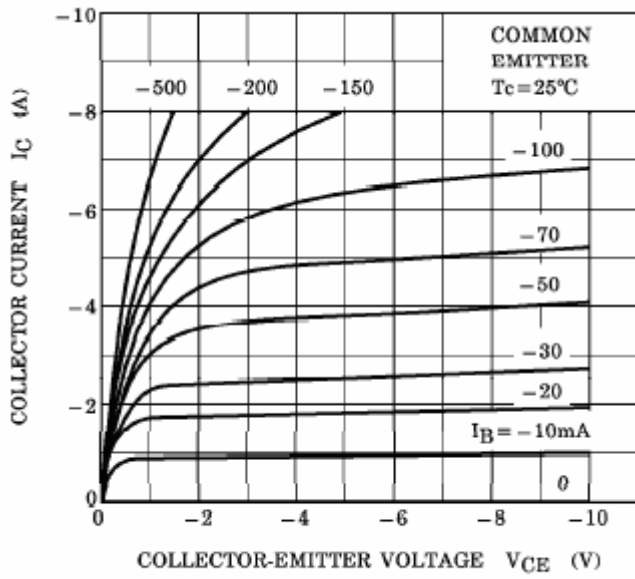
Fig.3 Static Characteristic
