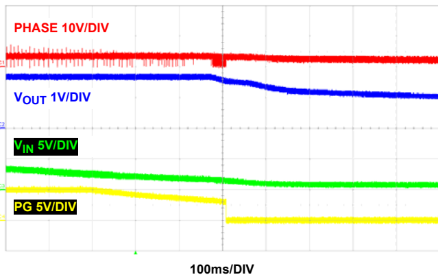
FIGURE 33. SHUTDOWN V_{IN} AT NO LOAD, PFM
