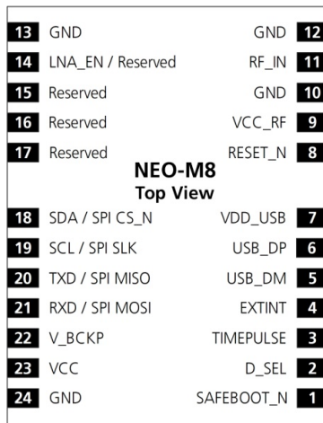
Figure 2: Pin assignment
