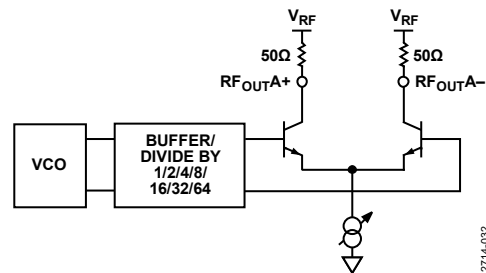
Figure 37. Output Stage
