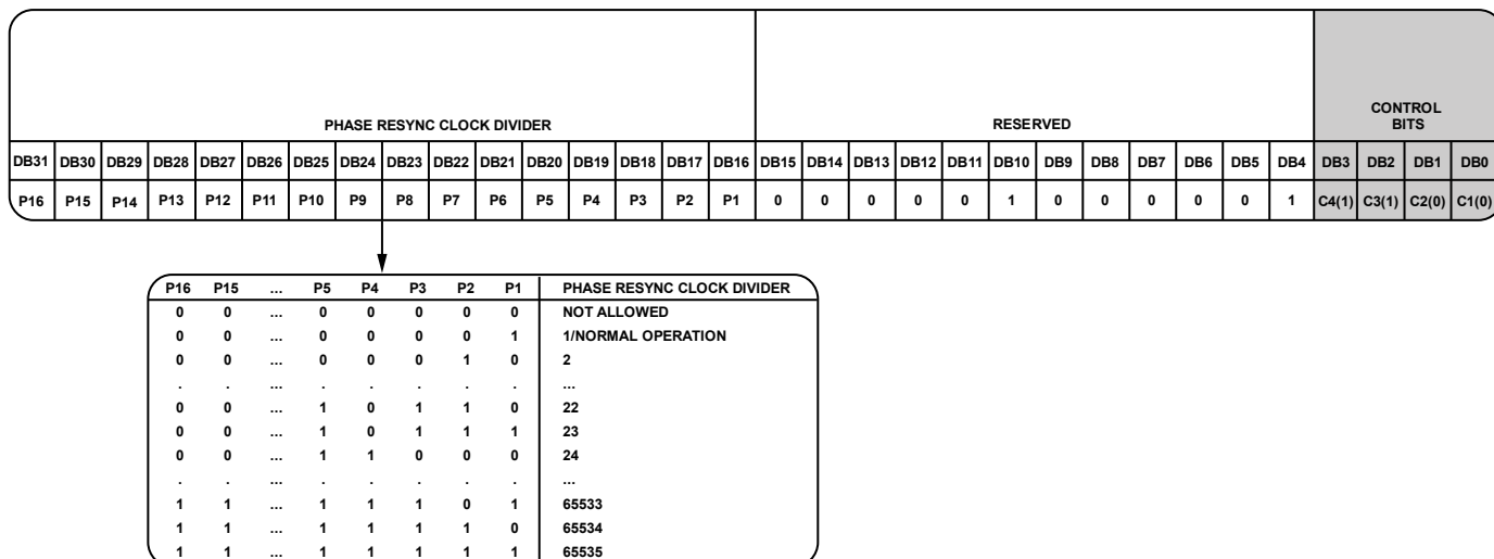
Figure 53. Register 12
