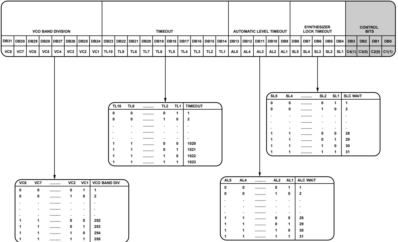
Figure 50. Register 9
