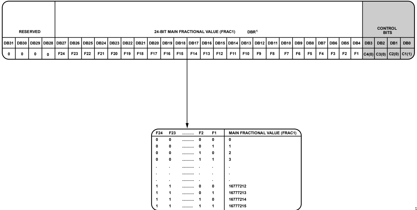
Figure 42. Register 1
