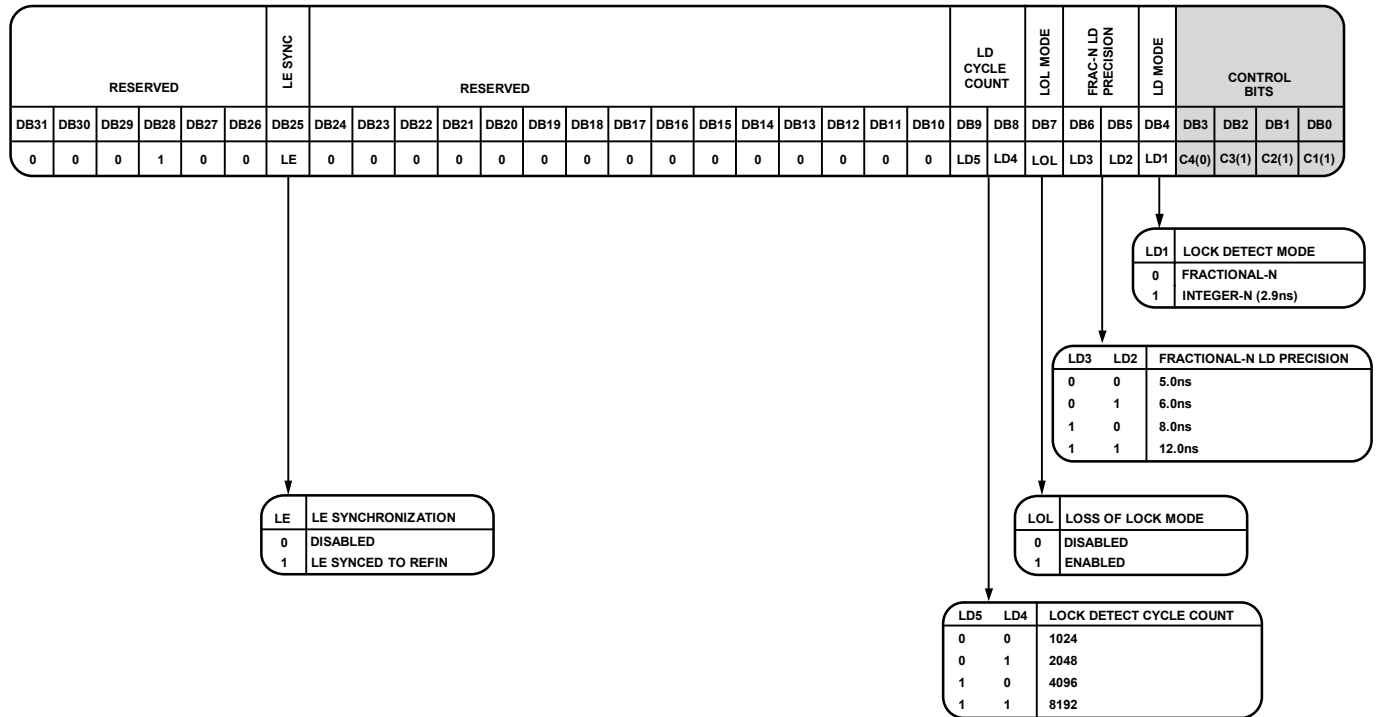
Figure 48. Register 7
