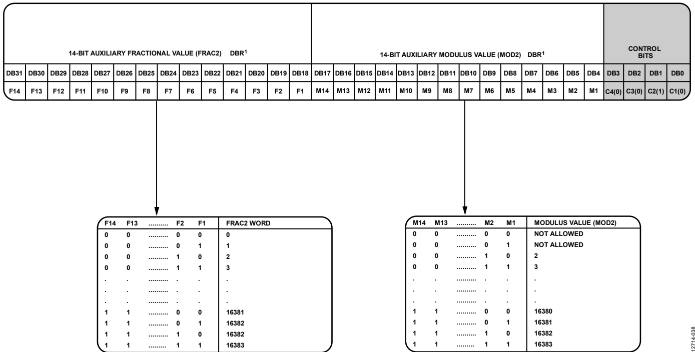
Figure 43. Register 2
