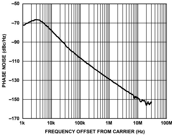
Figure 17. Closed-Loop Phase Noise, R_{F_{OUT}B} = 10 GHz, 2 \times VCO , VCO = 5.0 GHz, f_{PDF} = 61.44 MHz, Loop Bandwidth = 2 kHz
