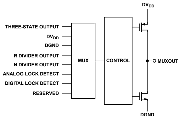
Figure 35. MUXOUT Schematic
