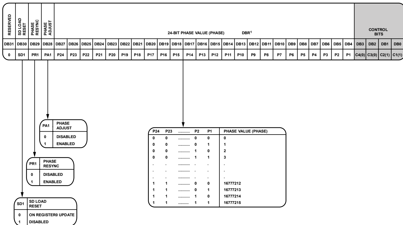
Figure 44. Register 3
