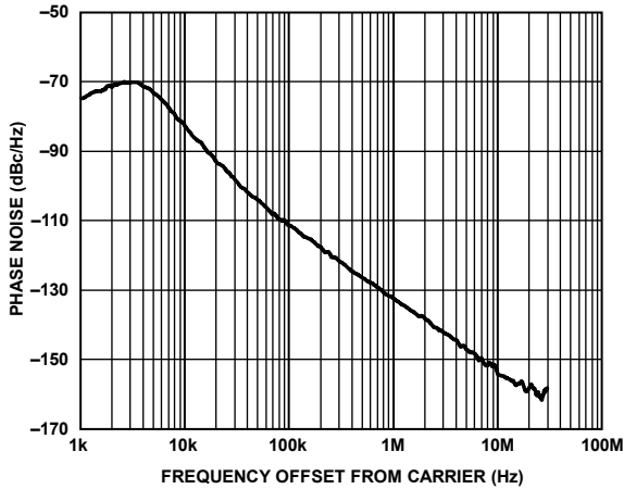
Figure 16. Closed-Loop Phase Noise, R_{F_{OUT}B} = 6.8 GHz, 2 \times VCO , VCO = 3.4 GHz, f_{PDF} = 61.44 MHz, Loop Bandwidth = 2 kHz
