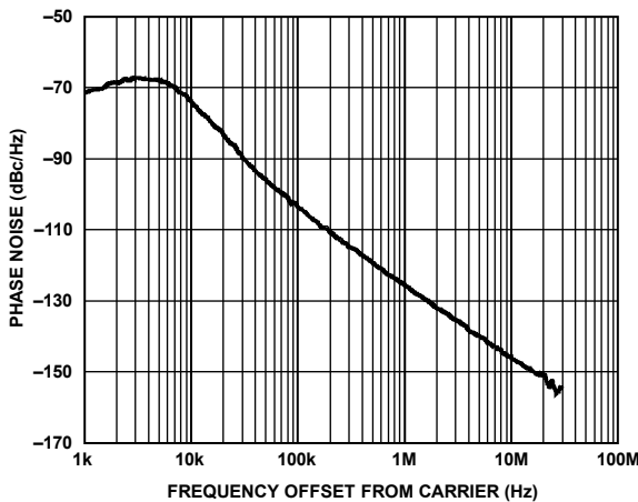
Figure 18. Closed-Loop Phase Noise, R_{F_{OUT}B} = 13.6 GHz, 2 \times VCO , VCO = 6.8 GHz, f_{PDF} = 61.44 MHz, Loop Bandwidth = 2 kHz
