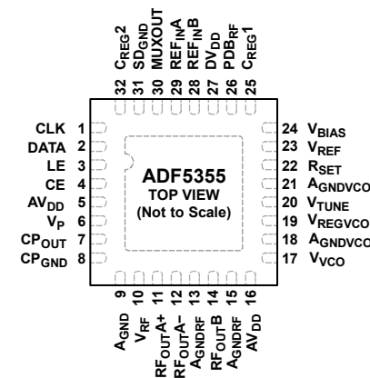
Figure 3. Pin Configuration
