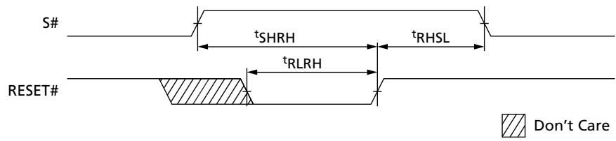
Figure 34: Reset AC Timing During PROGRAM or ERASE Cycle
