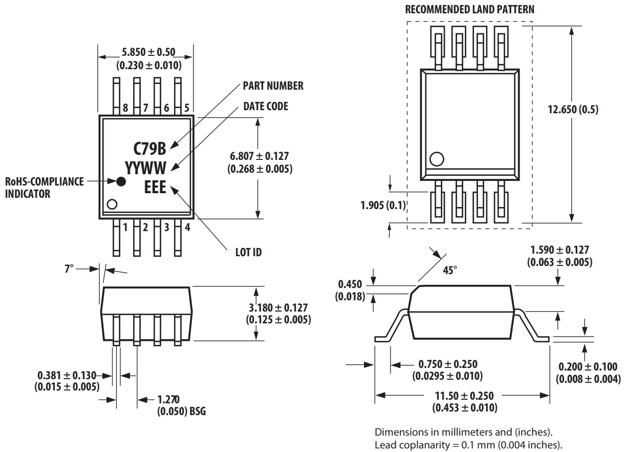
Figure 2. SS0-8 package.
