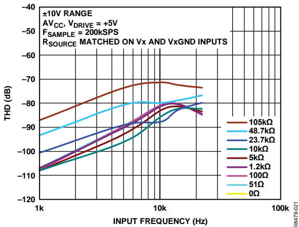
Figure 24. THD vs. Input Frequency for Various Source Impedances, ±10V Range
