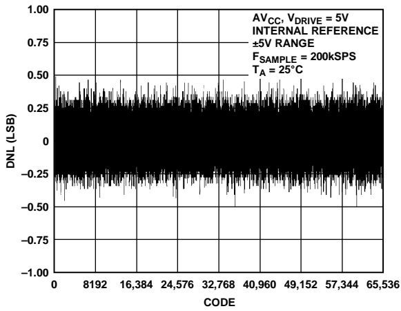
Figure 17. AD7606 Typical DNL, \pm 5V Range
