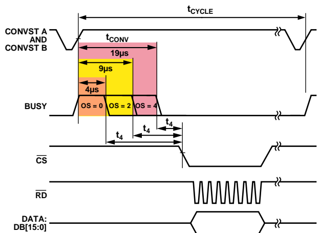
Figure 47. AD7606—No Oversampling, Oversampling × 2, and Oversampling × 4 While Using Read After Conversion
