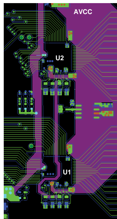
Figure 64. Layout for Multiple AD7606 Devices—Top Layer and Supply Plane Layer
