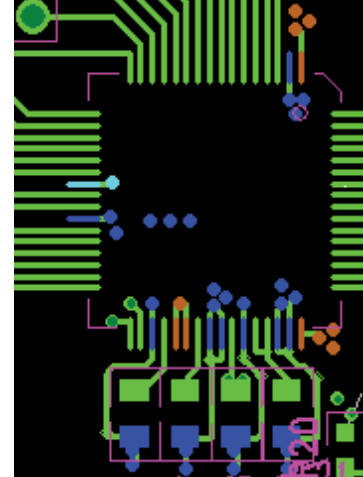
Figure 62. Top Layer Decoupling REFIN/REFOUT, REFCAPA, REFCAPB, and REGCAP Pins
