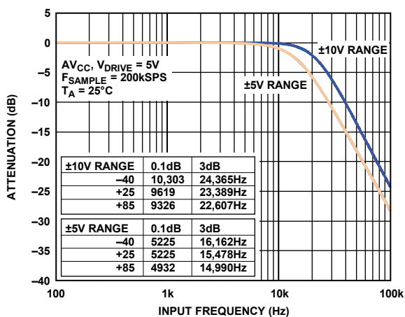
Figure 37. Analog Antialiasing Filter Frequency Response
