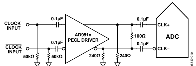
Figure 48. Differential PECL Sample Clock (Up to 4x Rated Sample Rate)
