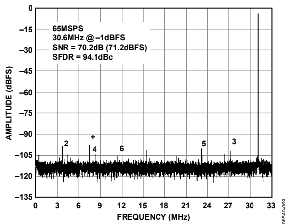
Figure 17. AD9629-65 Single-Tone FFT with f_{IN} = 30.6 MHz
