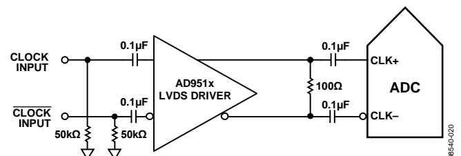
Figure 49. Differential LVDS Sample Clock (Up to 4x Rated Sample Rate)
