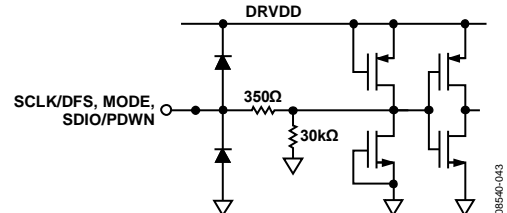
Figure 31. Equivalent SCLK/DFS, MODE, and SDIO/PDWN Input Circuit
