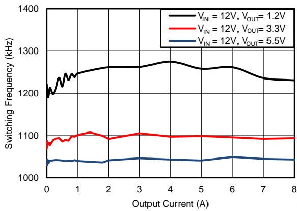
Figure 19. F_{SW} Load Regulation, Mode = FCCM, F_{SW} = 1200kHz
