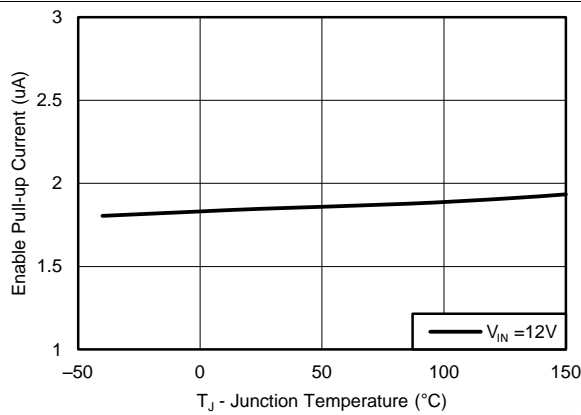
Figure 7. Enable Pull-up Current, V EN = 1.0V
