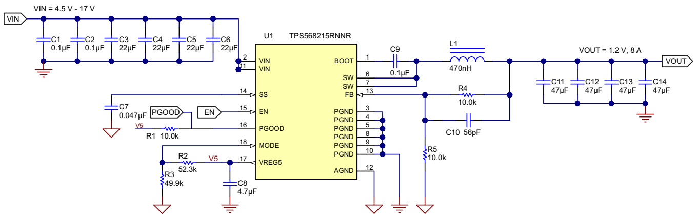
Figure 23. Application Schematic
