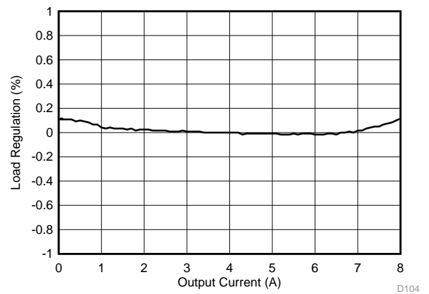
Figure 27. Load Regulation, V_{IN} = 12\text{ V}
