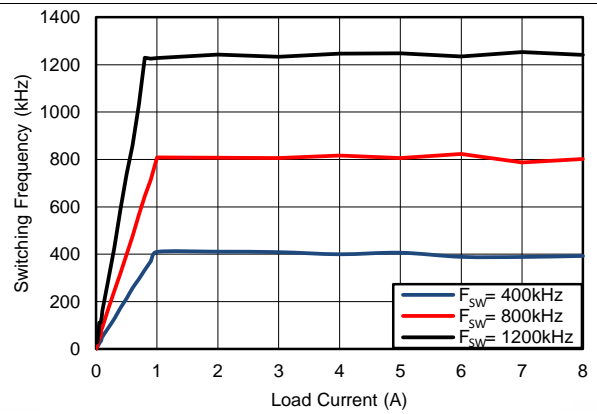
Figure 20. F_{SW} Load Regulation, Mode = DCM, V_{IN} = 12V, V_{OUT}=1.2V
