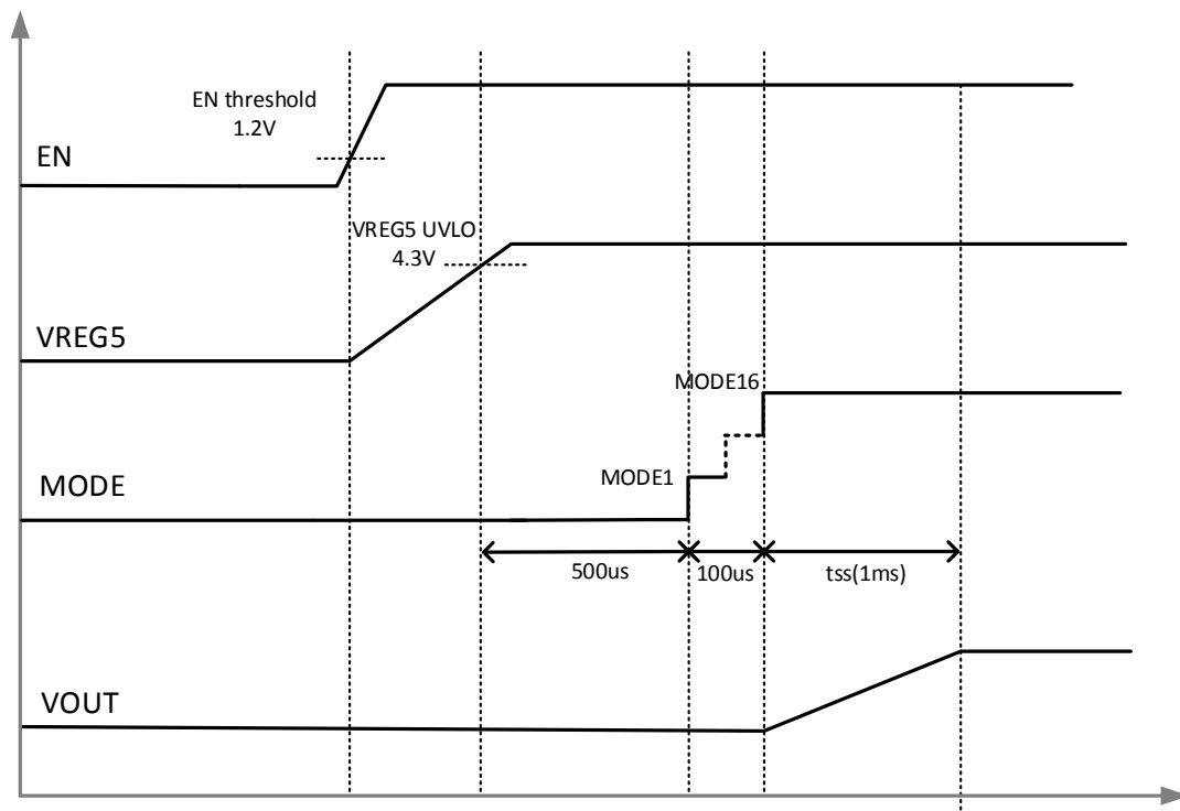
Figure 21. Power-Up Sequence
