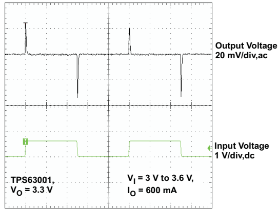
Timebase 2 ms/div V_O = 3.3\text{ V} V_I = 3\text{ V to }3.6\text{ V} I_O = 600\text{ mA}
