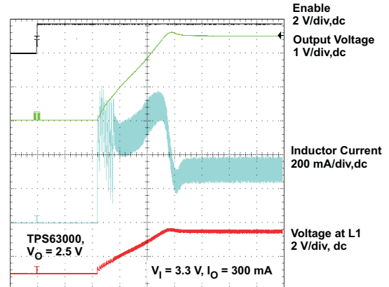
Timebase 50 \mu\text{s/div} V_O = 2.5\text{ V} V_I = 3.3\text{ V} I_O = 300\text{ mA}
