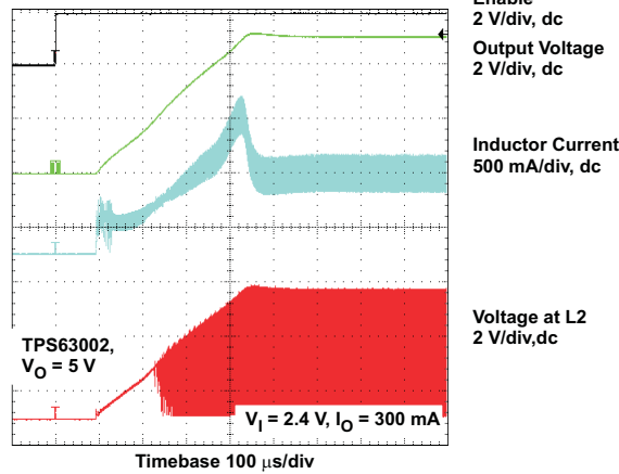
Timebase 100 \mu\text{s/div} V_O = 5\text{ V} V_I = 2.4\text{ V} I_O = 300\text{ mA}
