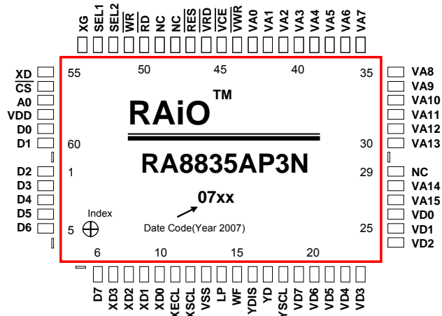
Figure 4-1: RA8835AP3N(QFP-60 Pin)
