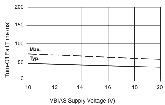
Figure 13B Turn-Off Fall Time vs. Voltage
