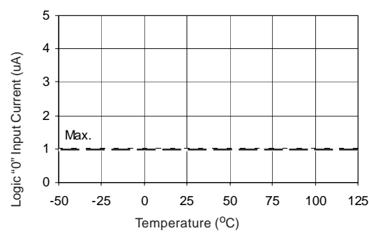
Figure 26A Logic "0" Input Current vs Temperature
