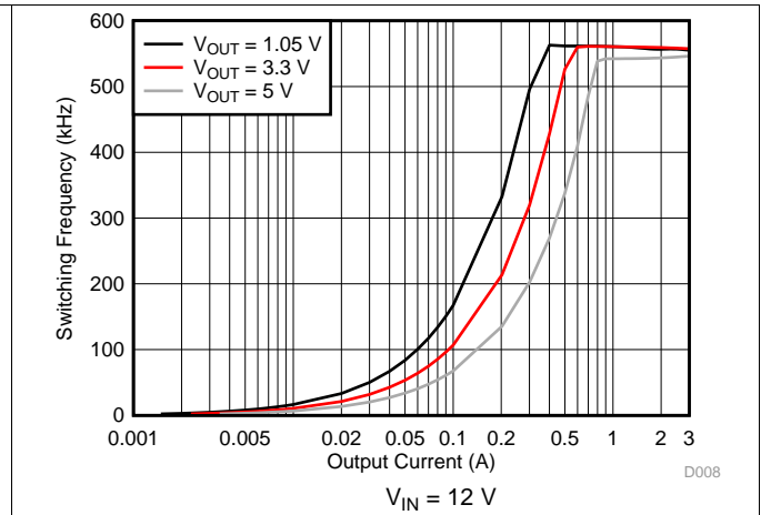
Figure 8. TPS563201 Switching Frequency vs Output Current
