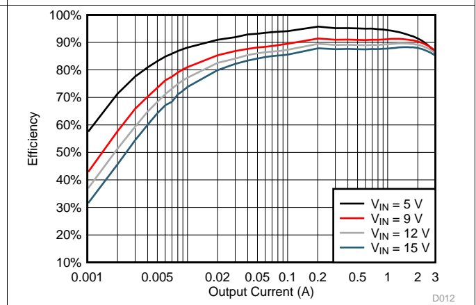
Figure 10. TPS563201 V_{OUT} = 1.5\text{ V} Efficiency, L = 2.2\ \mu\text{H}
