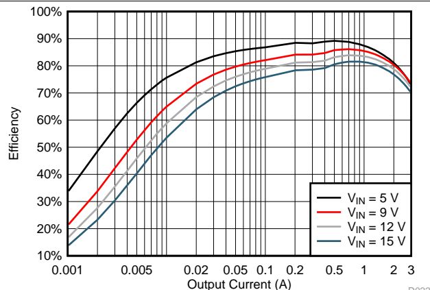
Figure 23. TPS563201 Efficiency
