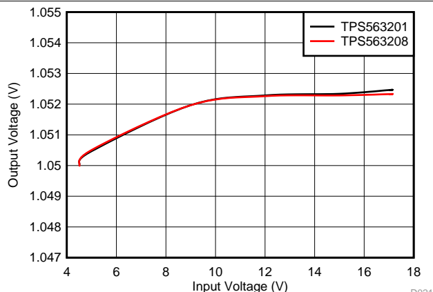
Figure 22. TPS563201 and TPS563208 Line Regulation
