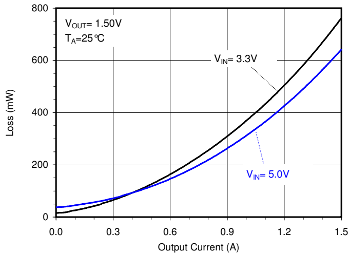
Total Loss vs. Load Current ( V_{OUT}=1.5\text{V} , SOT23-5)
