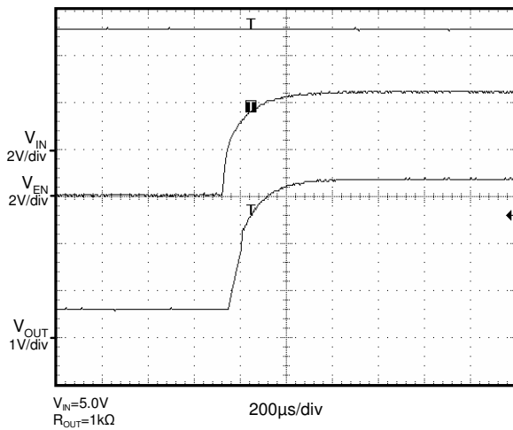
Start Up into Pre-Bias Output (Enable)
