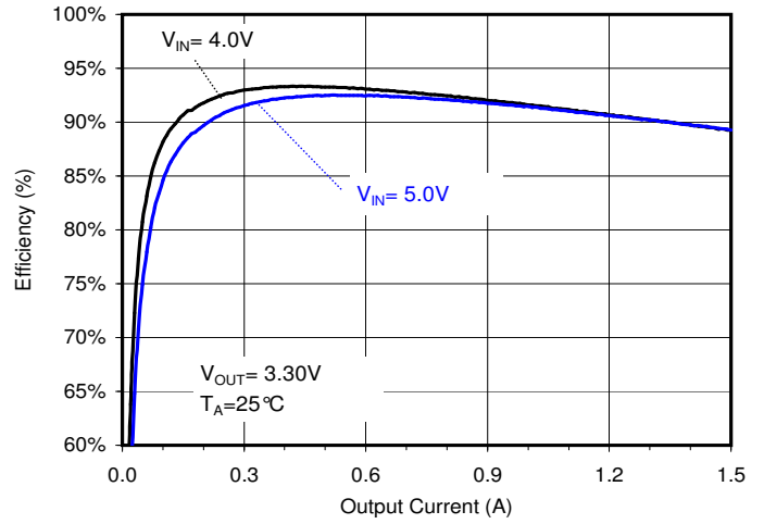
Efficiency vs. Load Current ( V_{OUT}=3.3\text{V} )
