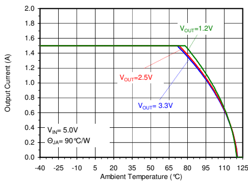
Figure 3 — Typical maximum output current over temperature of SOT23-5 package, V_{IN} = 5.0V
