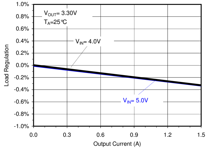
Load Regulation ( V_{OUT}=3.30\text{V} )
