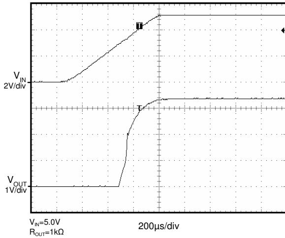
Start Up (Power up V_{IN} ) ( V_{OUT}=3.3V )
