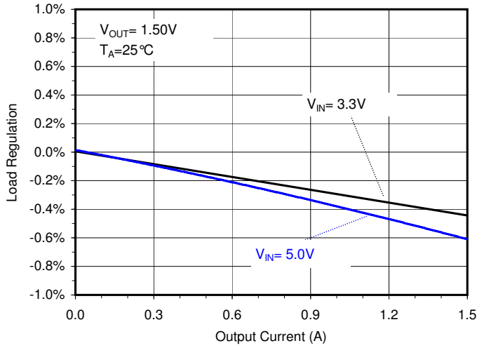
Load Regulation ( V_{OUT}=1.50\text{V} )
