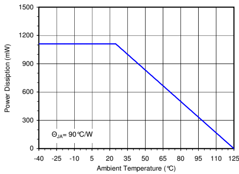
Figure 2 — Maximum power dissipation of SOT23-5 package over temperature
