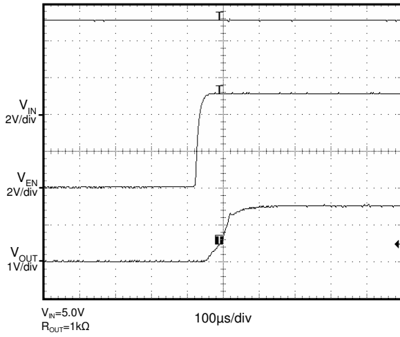
Start Up (Enable) ( V_{OUT}=1.5V )
