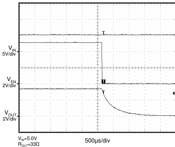
Shutdown (Disable) ( V_{OUT}=3.3V )
