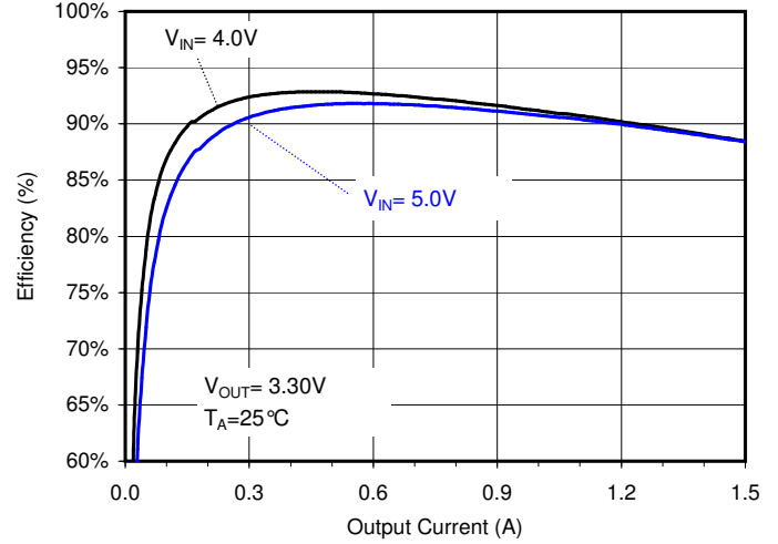
Efficiency vs. Load Current (SOT23-5)
