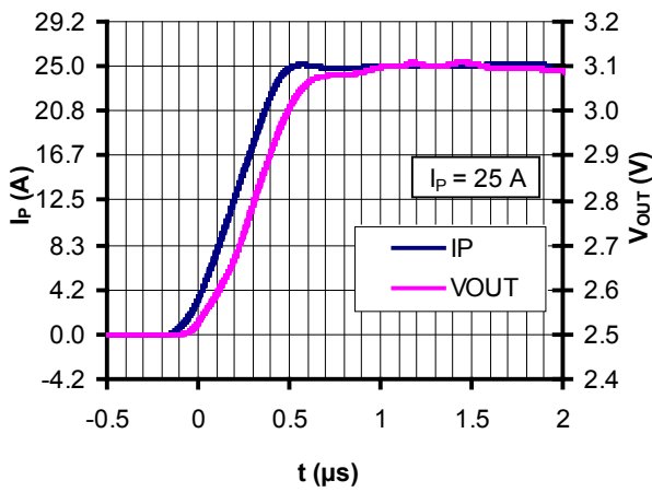
Figure 15: Step response
