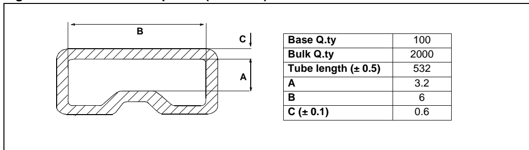
Figure 45. SO-8 tube shipment (no suffix)
