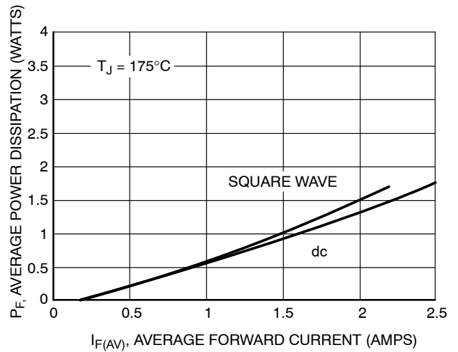
Figure 8. Power Dissipation
