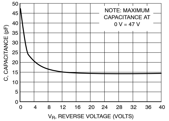
Figure 6. Maximum Capacitance
