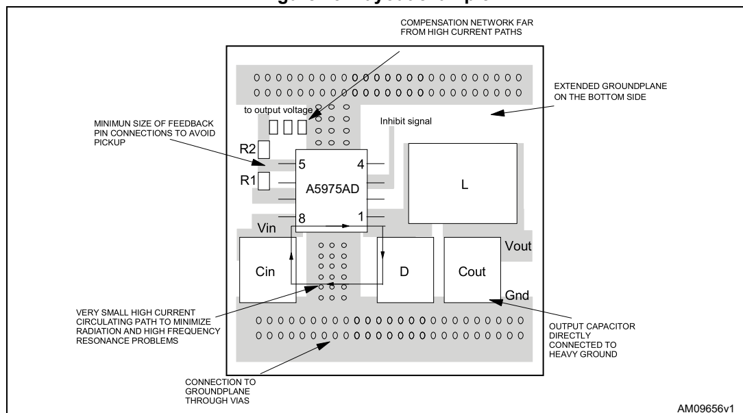
Figure 13. Layout example
