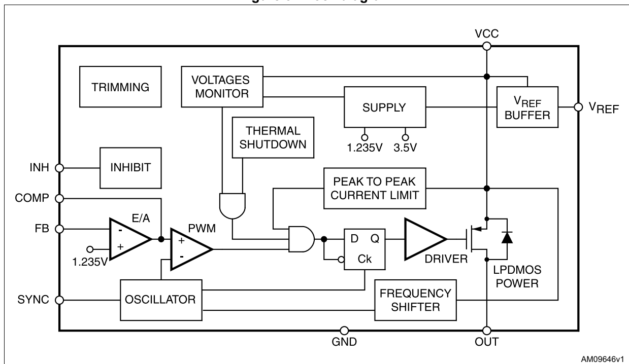
Figure 3. Block diagram
