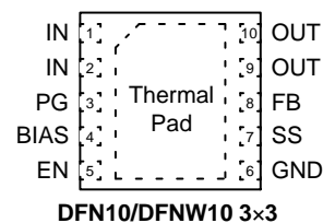
DFN10/DFNW10 3x3
