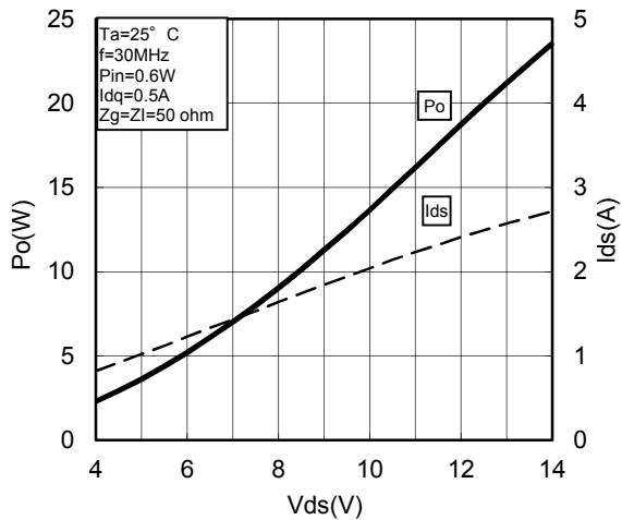
Vds-Po CHARACTERISTICS
