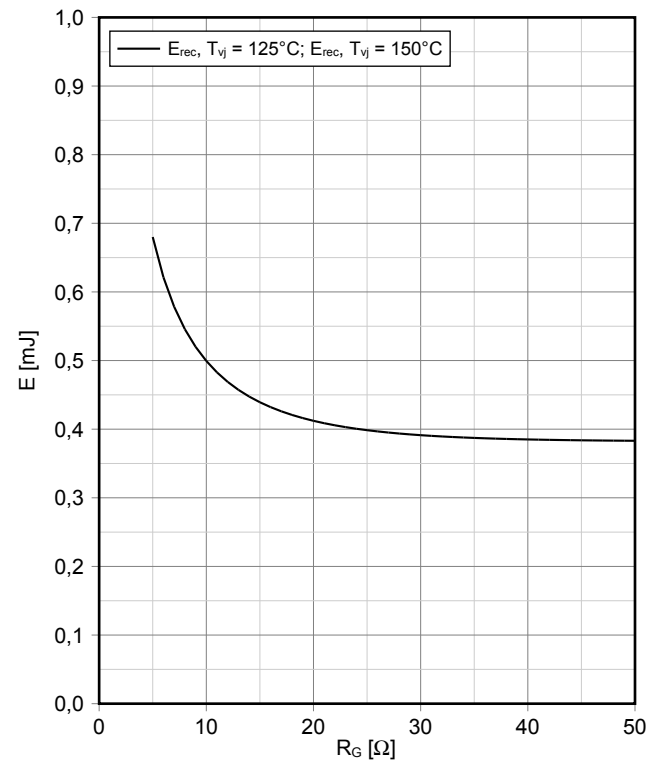
开关损耗 二极管, D5-D6 (典型) switching losses Diode, D5-D6 (typical) E_{rec} = f(R_G) I_F = 100 A, V_{CE} = 500 V
