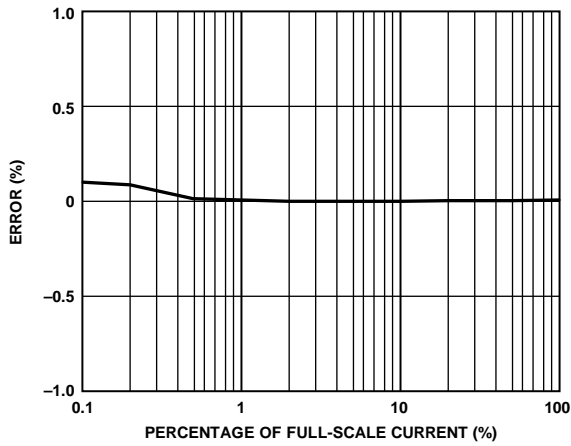
Figure 42. 10 Cycle Current RMS/12 Cycle Current Error, Gain = 4, Integrator On, Data Sourced After High-Pass Filter, Register CONFIG0, Bit RMS_SRC_SEL = 0
