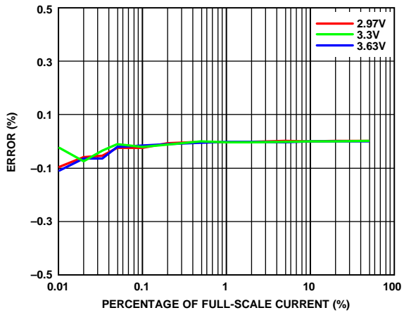
Figure 14. Fundamental Reactive Energy Error as a Percentage of Full-Scale Current over Supply Voltage, Power Factor = 0, T_A = 25^\circ\text{C}
