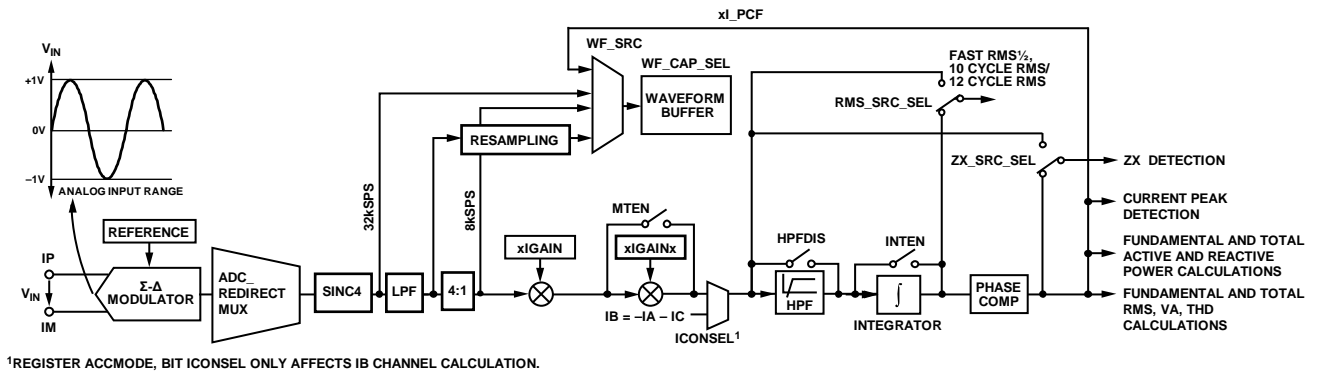
Figure 56. Current Channel (IA, IB, IC) Datapath
