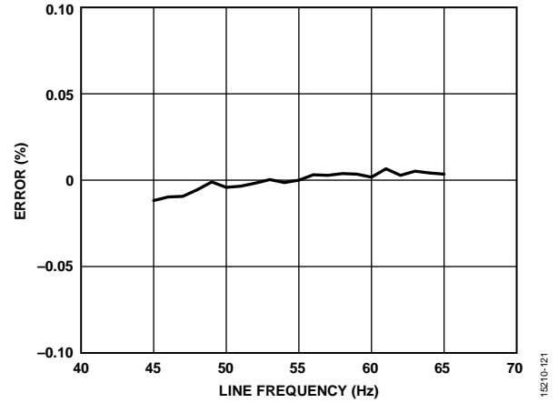
Figure 34. 1/2 Cycle Current RMS Error vs. Line Frequency, Data Sourced After High-Pass Filter, Register CONFIG0, Bit RMS_SRC_SEL = 0
