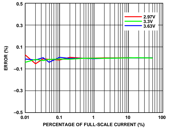
Figure 15. Fundamental Apparent Energy Error as a Percentage of Full-Scale Current over Supply Voltage, Power Factor = 1, T_A = 25^\circ\text{C}
