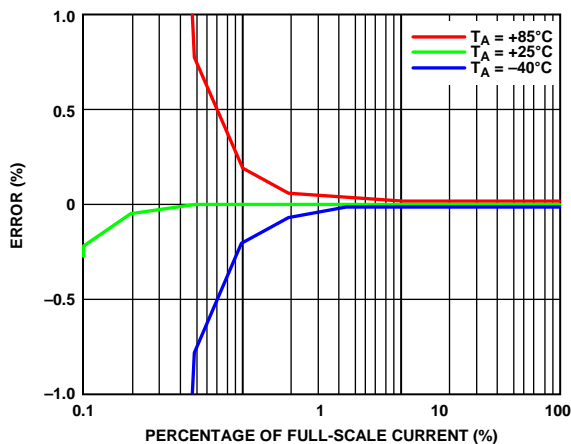
Figure 27. 1/2 Cycle Current RMS Error as a Percentage of Full-Scale Current over Temperature, Data Sourced Before High-Pass Filter and Calibrated for Offset, Register CONFIG0, Bit RMS_SRC_SEL = 1
