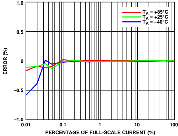
Figure 26. Current RMS Error as a Percentage of Full-Scale Current over Temperature
