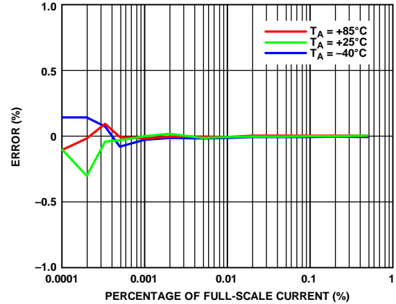
Figure 29. Fundamental Current RMS Error as a Percentage of Full-Scale Current over Temperature
