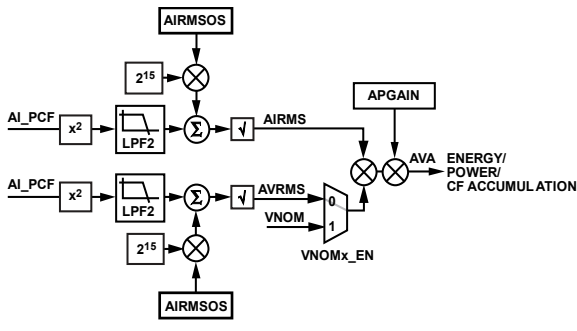
Figure 64. Total Apparent Power, AVA, Calculation for Phase A
