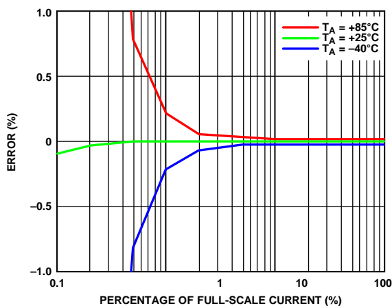
Figure 28. 10 Cycle Current RMS/12 Cycle Current Error as a Percentage of Full-Scale Current over Temperature, Data Sourced Before High-Pass Filter and Calibrated for Offset, Register CONFIG0, Bit RMS_SRC_SEL = 1
