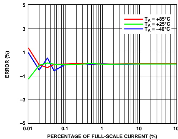
Figure 30. 1/2 Cycle Current RMS Error as a Percentage of Full-Scale Current over Temperature, Data Sourced After High-Pass Filter, Register CONFIG0, Bit RMS_SRC_SEL = 0
