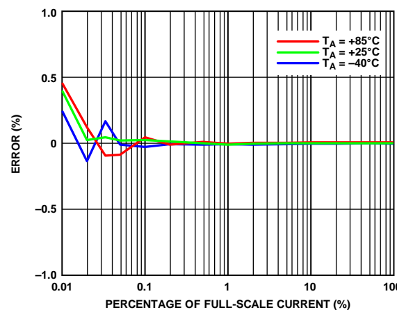
Figure 31. 10 Cycle Current RMS/12 Cycle Current Error as a Percentage of Full-Scale Current over Temperature, Data Sourced After High-Pass Filter, Register CONFIG0, Bit RMS_SRC_SEL = 0
