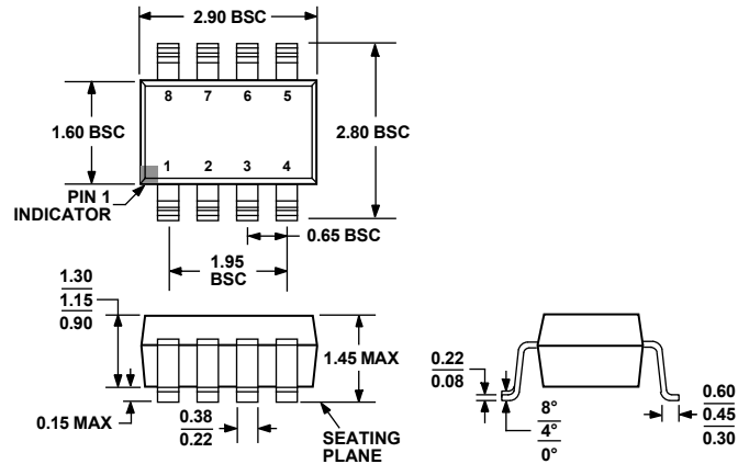
COMPLIANT TO JEDEC STANDARDS MO-178-BA Figure 48. 8-Lead Small Outline Transistor Package [SOT-23] (RJ-8) Dimensions shown in millimeters
