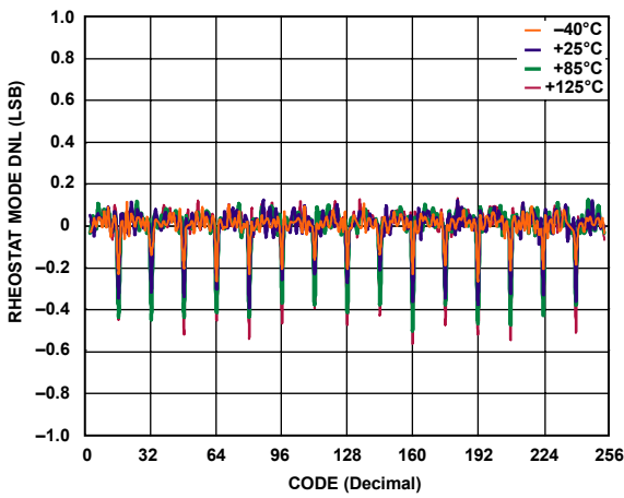
Figure 11. R-DNL vs. Code vs. Temperature, V_{DD} = 5\text{ V}
