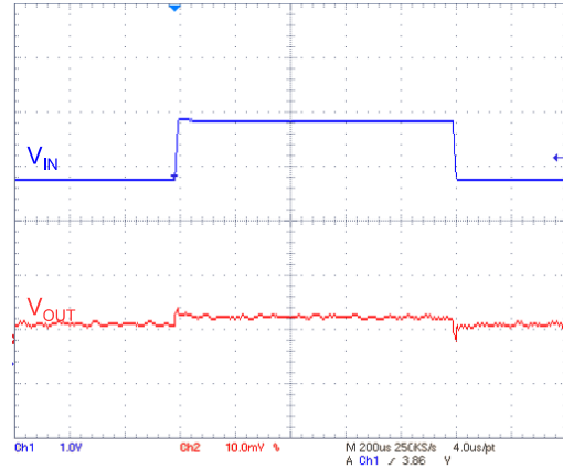
Figure 23: Line transient (I OUT = 250 mA)
