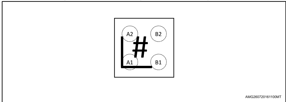
Figure 35: Flip-Chip marking composition (marking view)
