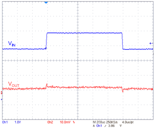
Figure 22: Line transient (I OUT = 1 mA)
