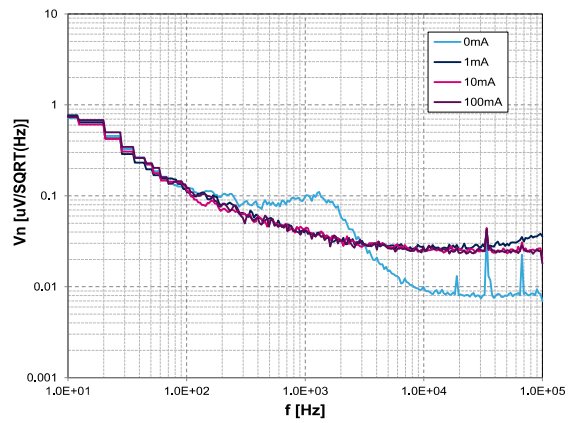
Figure 21: Noise density
