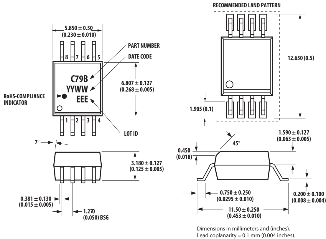
Figure 2: SSO-8 Package
