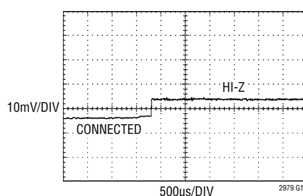
DAC Soft-Connect Transient Response When Transitioning from ON State to Hi-Z State
