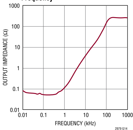
DAC Output Impedance vs Frequency
