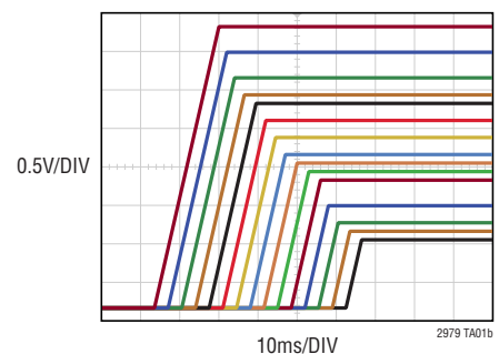
LTC2979 Sequencing 16 Channels
