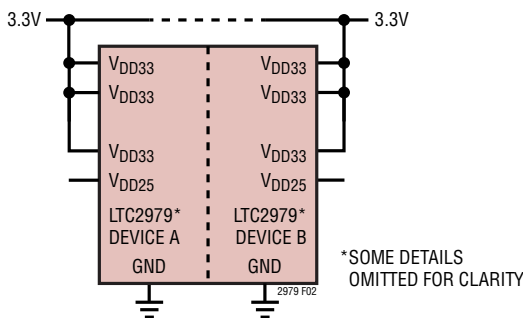
Figure 2. Powering LTC2979 from a 3.3V Supply
