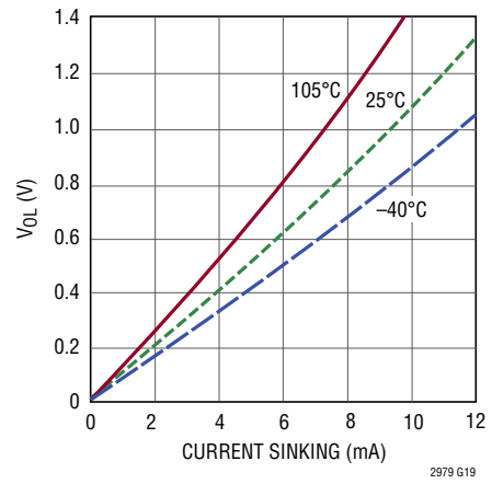
V_{OUT\_EN[3:0]} and V_{IN\_EN} Output V_{OL} vs Current
